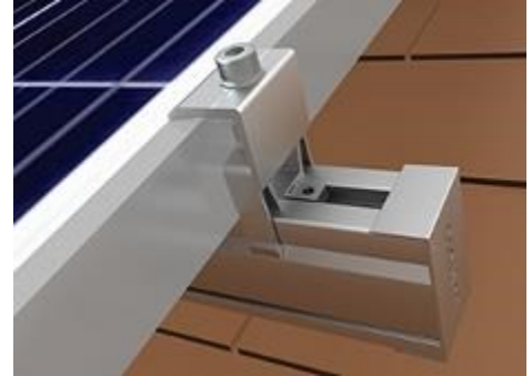
Pop-On End Clamps are adjustable for different module frame heights and provide fast and secure attachment of modules.
