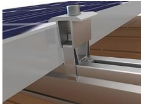
The Bonding Pop-On Universal Mid Clamps accommodate PV module frame heights ranging from 30mm to 50mm.
